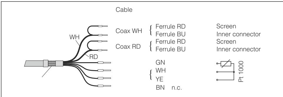
10 Fixed cable/special measuring cable CLK6
