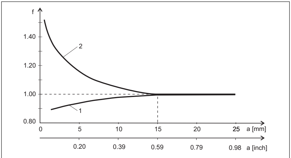
5 Relationship between installation factor f and wall distance a
