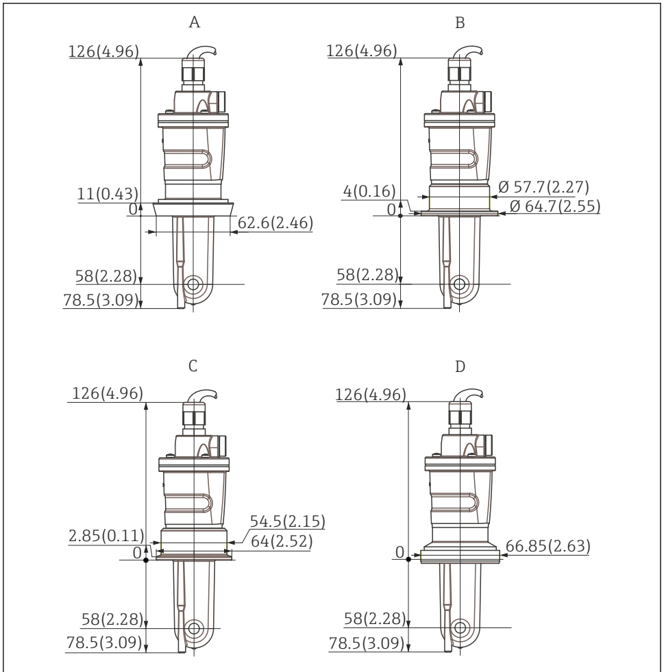
9 Process connections for CLS54 (long version), dimensions in mm (inch)
