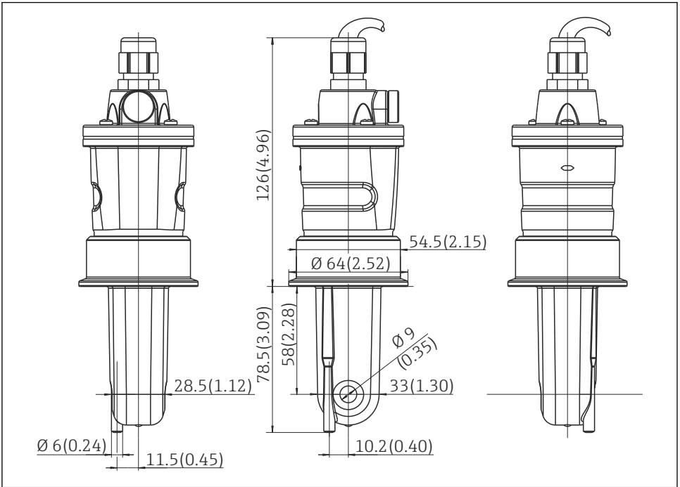
7 Dimensions in mm(inch) (long version)
